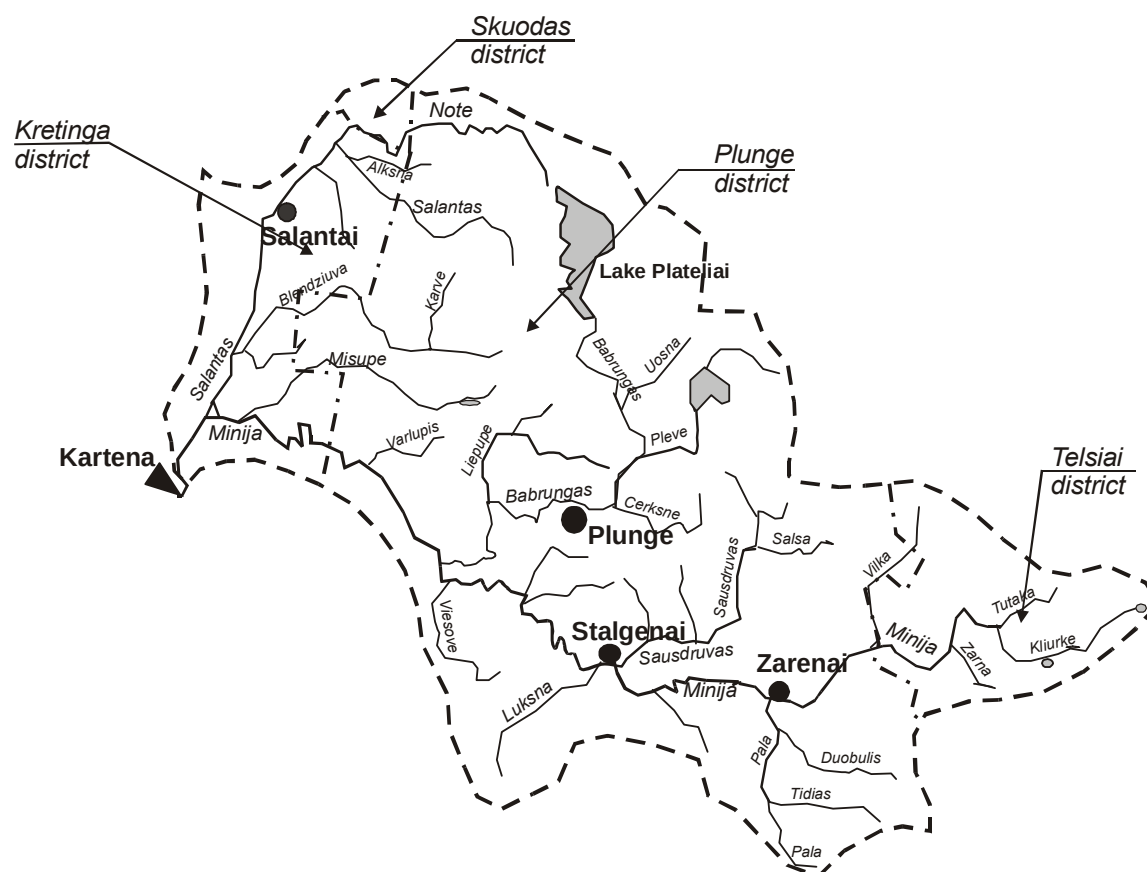
Figure 1. Scheme of the Minija_Kartena catchment.
