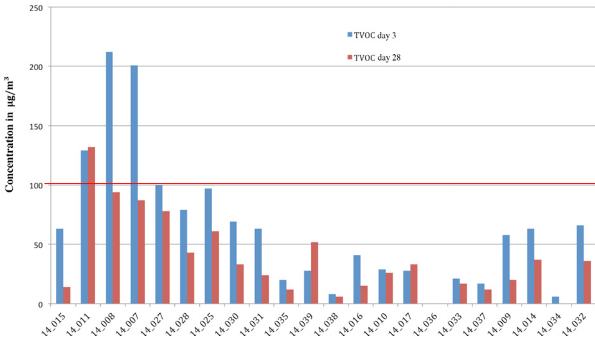
Figure Z2: TVOC values of the AgBB evaluation of the textile floor coverings on day 3 and 28 (red line: limit value on day 28 UZ 128 = 100 µg/m³) [Source: own illustration, BAM]
