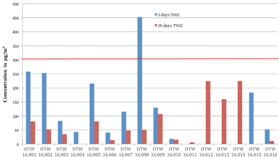
Figure Z5: TVOC values of the AgBB evaluation of the elastic floor coverings on the days 3 and 28 (red line: limit value UZ 120 = 300 \mu\text{g}/\text{m}^3 ) [Source: own illustration, BAM]
