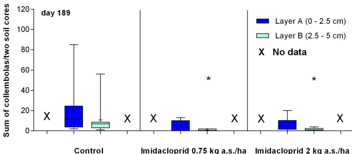
Figure 56 Total abundance of collembolans in the soil layers of the TMEs in study [1] (10 replicates for control; 5 replicates for imidacloprid treatments). X: no data; cross: mean; *: significance (p-value Williams-test < 0.05). Sampling dates at day 14 - 364 from top to bottom
