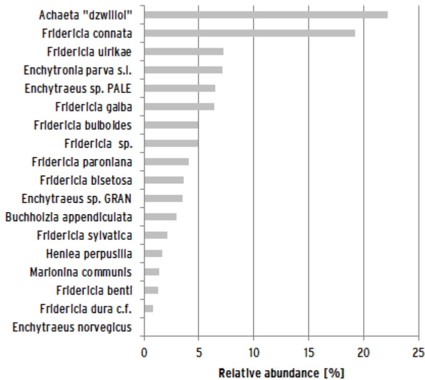
Figure 35 Dominance spectrum of echytraeids over all sampling dates in the control TMEs (n=10).
