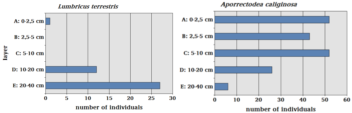
Figure 53 Vertical distribution of the lumbricid species Lumbricus terrestris and Aporrectodea caliginosa in the control. Shown is the total number of individuals captured in all TMEs on all sampling dates in the study [1].
