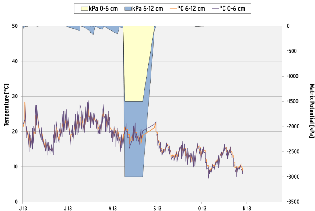
Figure 77 Data from continuous measurement of equitensimeter and temperature sensors in the study [3] from June 2013 to November 2013.
