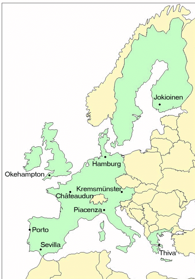
Figure 99 Locations of the FOCUS groundwater scenarios
