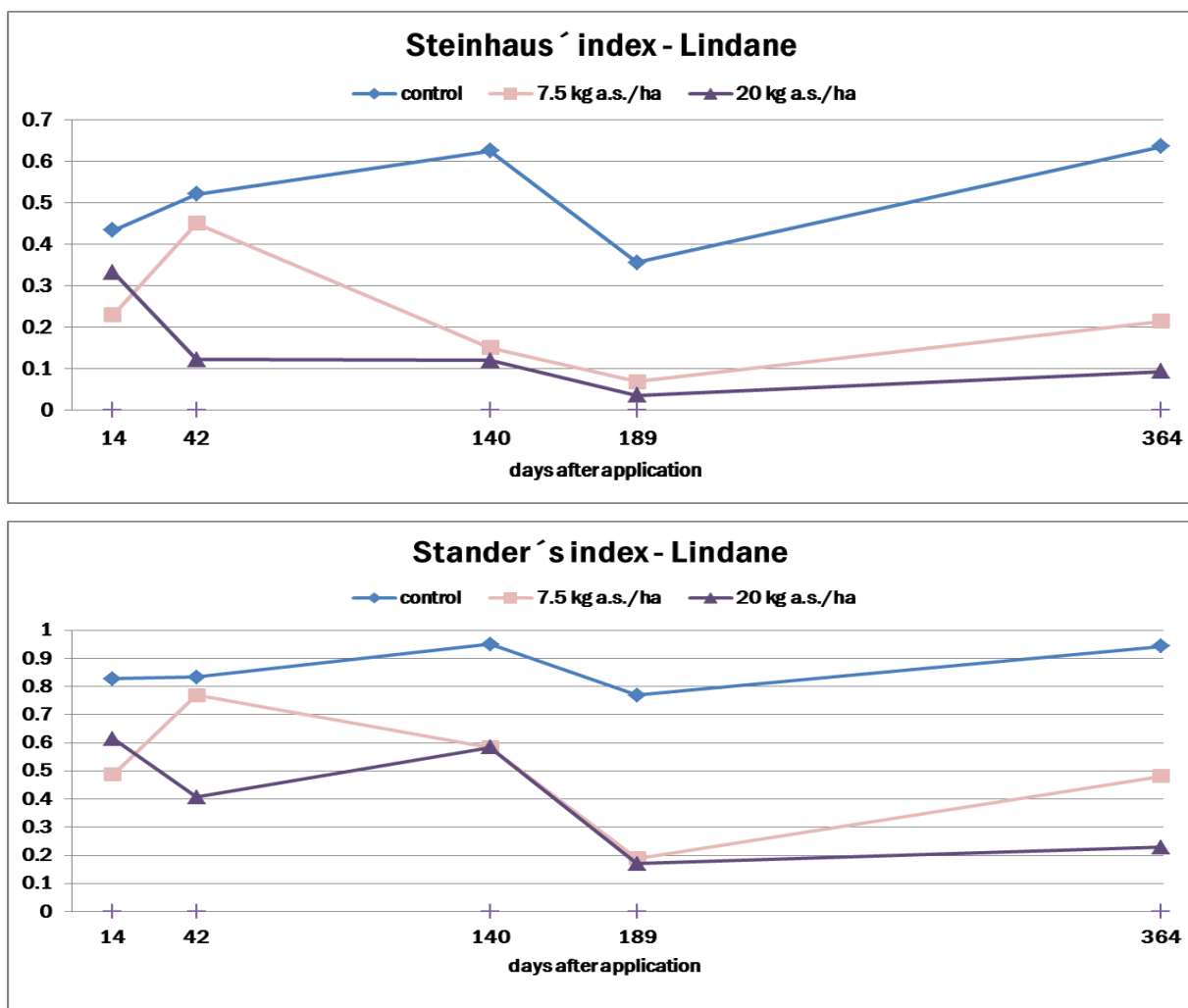
Figure 46 Similarity of oribatid mite diversity summed up over soil layers A-C (above) Steinhaus index (below) Standers index. Calculation is based on 10 replicates for the control and 5 replicates for each treatment.
