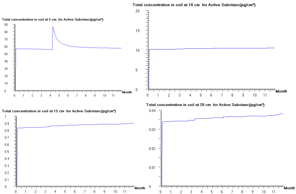
Figure 102 Lindane concentrations in soil at Kremsmünster calculated with PELMO 553 based on parameters obtained by inv. modelling (grass/alfalfa, annual application of 16.3 kg/ha)
