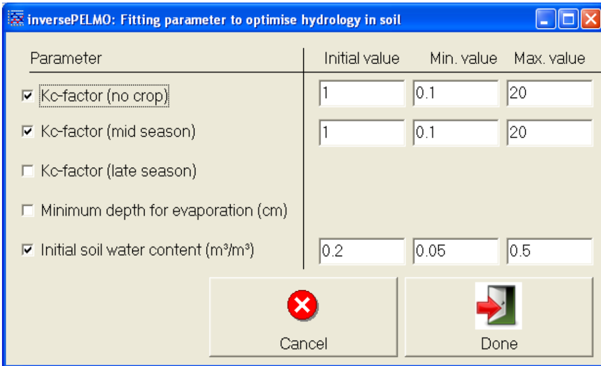
Figure 89 Parameters used in the optimisation of the leachate (TME study 1)
