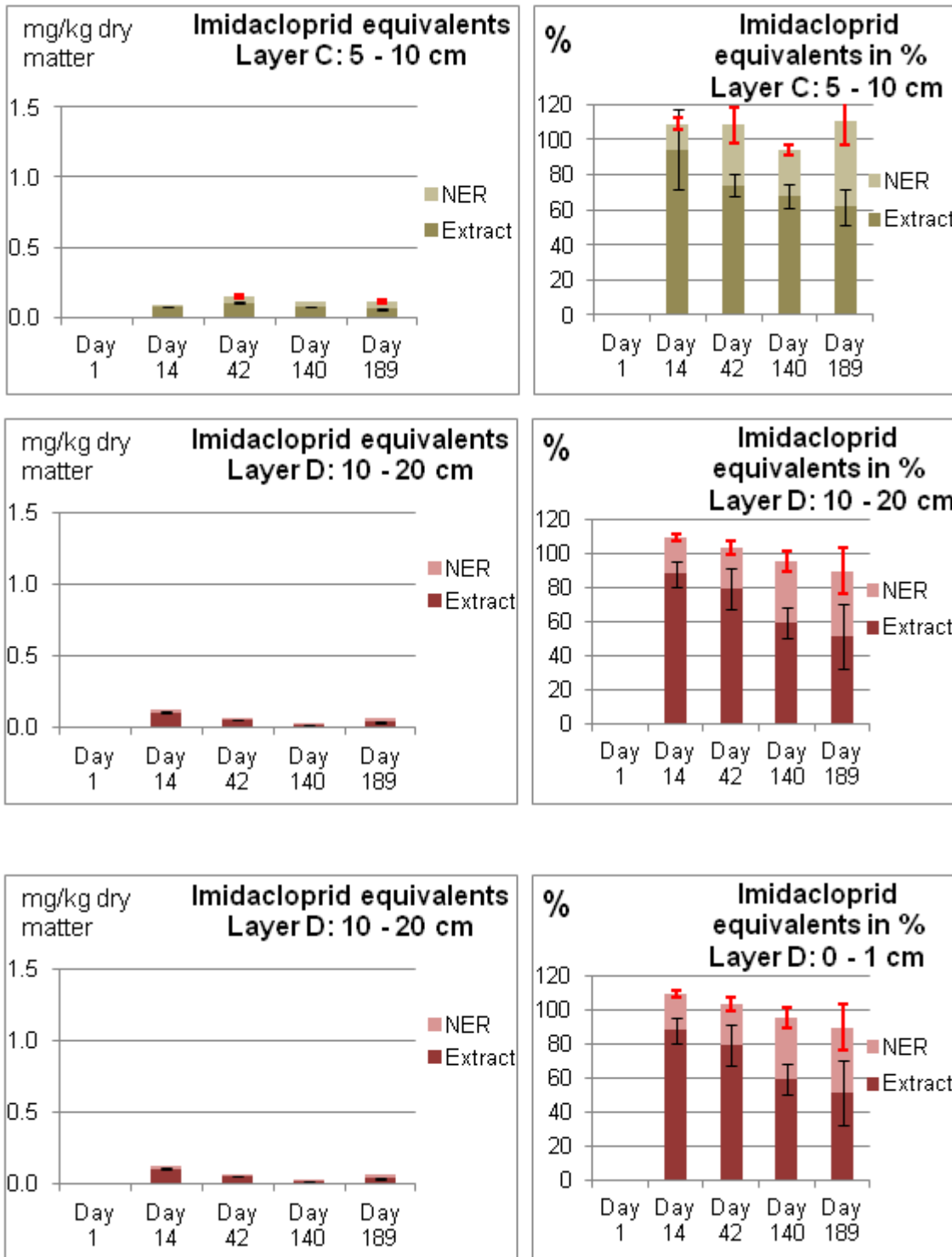
Figure 74 In the left figure the concentration of Imidacloprid equivalents in soil dry matter are given in mg/kg for the respective layer. Error bars indicating the standard deviation. The right figure show the percentage of the Imidacloprid equivalents of the extractable and the non-extractable residues referring to the total amount of Imidacloprid. This total amount was measured after the combustion of the non-extracted soil sample.
