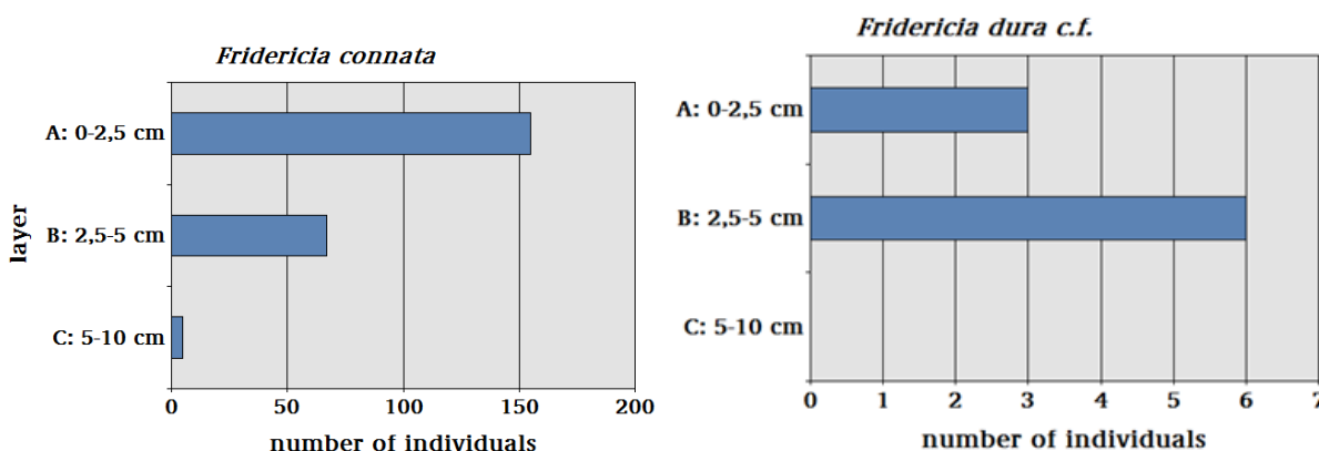
Figure 64 Vertical distribution of the enchytraeid species Fridericia connata and Fridericia dura c.f. in the control. Shown is the total number of individuals captured in all soil cores on all sampling dates.
