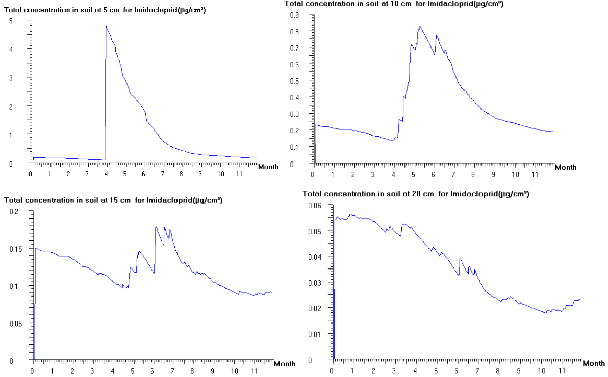
Figure 110 Imidacloprid concentrations in soil at Kremsmünster calculated with PELMO 553 based on parameters obtained by inv. modelling (grass/alfalfa, annual application of 2.38 kg/ha)
