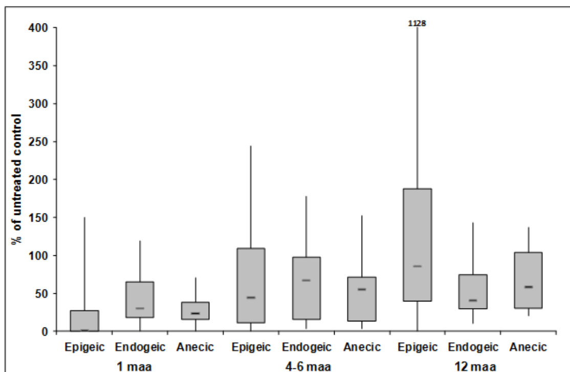
Figure 3 Boxplots of the relative abundance of the three ecological groups of earthworms at 16 grasslands treated with Benomyl or Carbendazim compared to the untreated control (maa = months after application) (Römbke et al. 2010).
