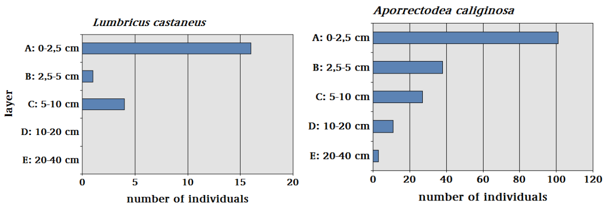
Figure 83 Vertical distribution of the lumbricid species Lumbricus castaneus and Aporrectodea caliginosa in the control. Shown is the total number of individuals captured in all TMEs on all sampling dates in the study [3].
