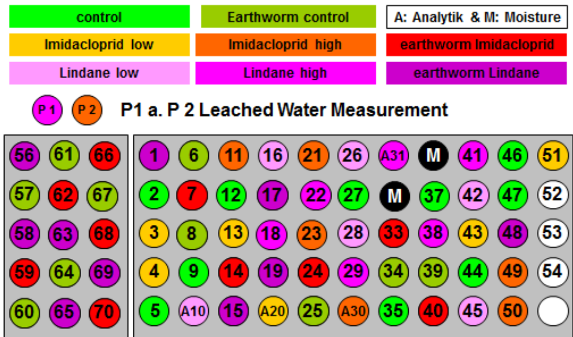
Figure 9 Randomised study design with controls, two pesticides (Lindane & Imidacloprid) in two application rates each and measurement of leachate water. The TMEs named control, Imidacloprid low/high and Lindane low/high were used to sample microarthropods and enchytraeids. Analytical measurement for the pesticide in the soil layers 0-2.5 cm; 2.5-5 cm and 5-10 cm were also taken within these TMEs. The “earthworm”-TMEs were used for sampling earthworms only. The four TMEs labelled with A were considered to measure the pesticide concentrations in deeper soil layers 10-20 cm
