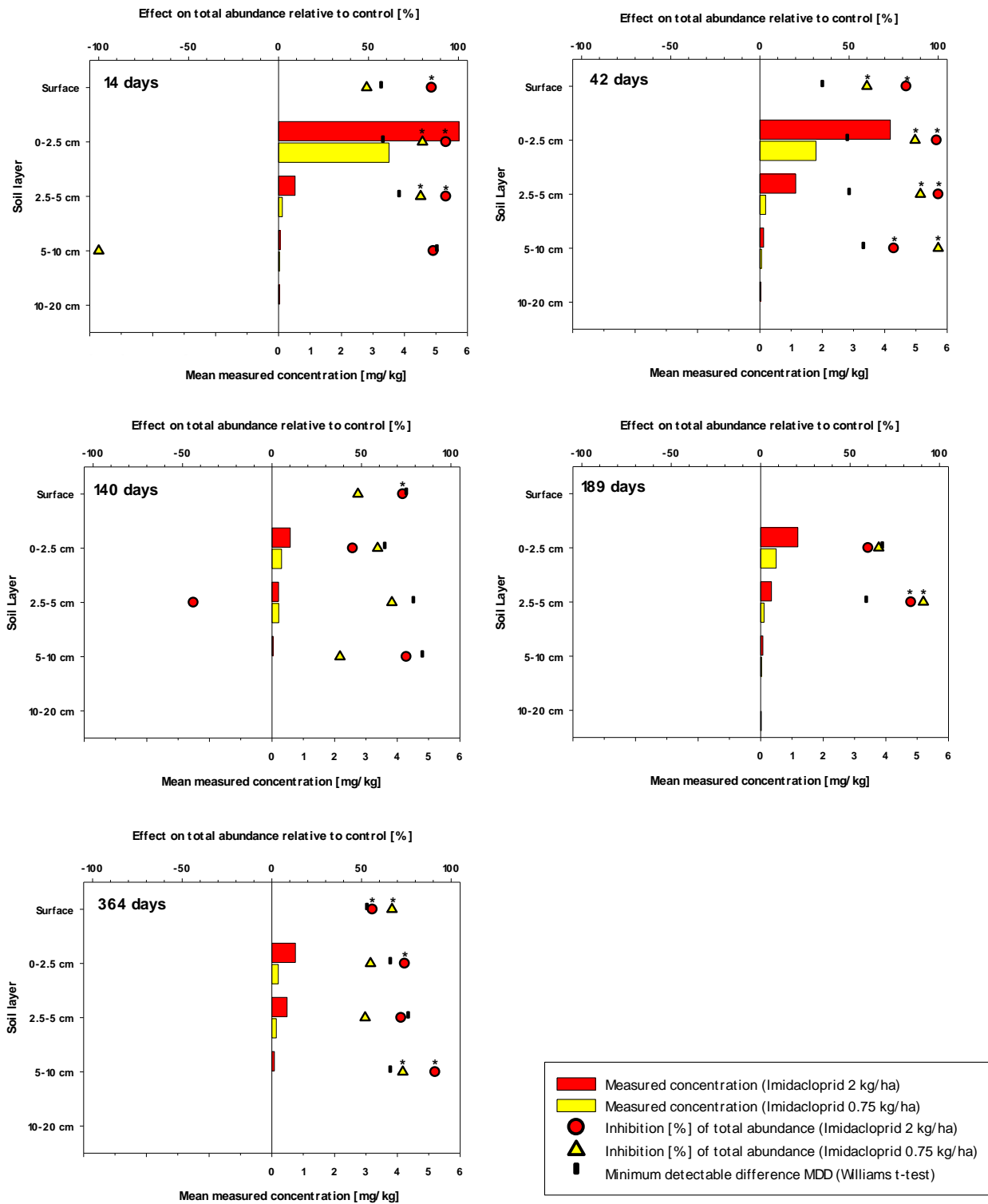
Figure 122 Decrease of total abundance of Collembolan species in the Imidacloprid-treatments 0.75 kg a.s./ha and 2.0 kg a.s. /ha (5 replicates each) for the different soil layers in comparison to the control (10 replicates). Columns showing the measured concentration for the two treatment concentrations at the respective sampling date. *: significant difference according to Williams t-test; bars showing the minimum detectable difference (MDD) as value for the specific possible statistical resolution. MDD values higher than 100 % are not shown.
