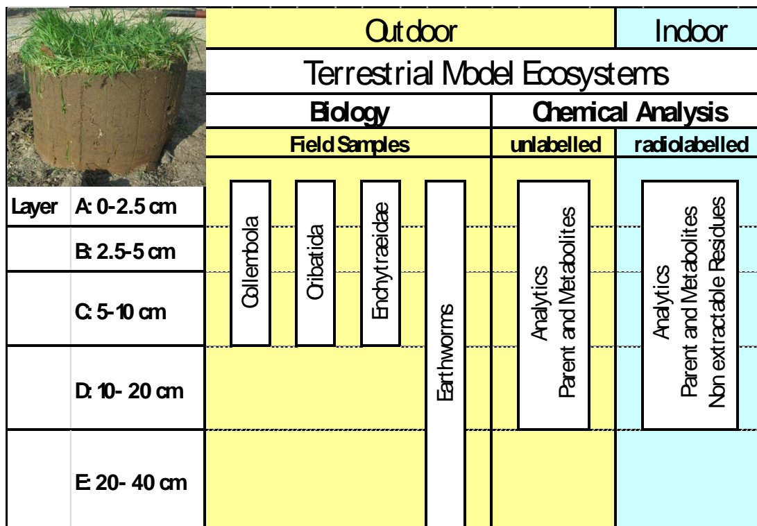
Figure 10 Link of analytical and biological data out of the field (outdoor study [1] and indoor laboratory study [2] by sampling in Terrestrial Model Ecosystems (TMEs).
