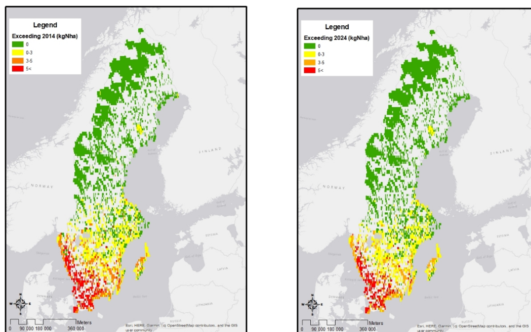
Figure 34 Exceedance CL emp N 2014 submission (left) and CL emp N 2024 submission (right) using N-deposition from EMEP for year 2018. Using the CL emp N submitted by Sweden in 2014 the CL was (deposition year 2018) exceeded at 14.9% N2000 area, which is essentially the same outcome as the current submission (14.4% area exceedance).
