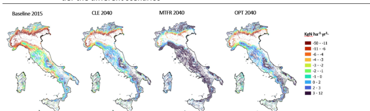
Figure 21 Exceedances calculated with respect to the CL_{emp} minimum value of the range under the different scenarios
