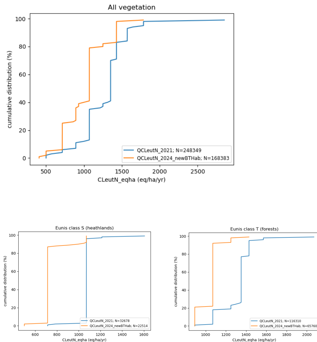
Figure 40 Cumulative frequencies of CLeutN in eq.ha-1.yr-1 for all vegetations (a) and for heathlands and forest separately (b,c) for the 2021 and the current submission.
