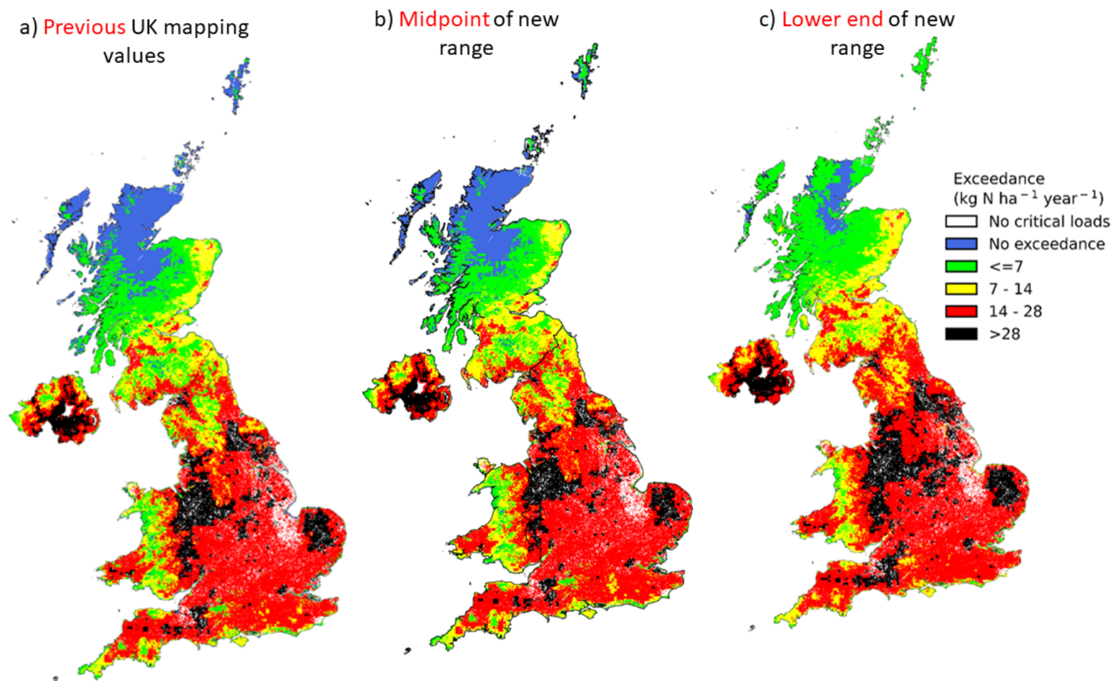
Figure 36 Excess Nitrogen (Average Accumulated Exceedance of nutrient-nitrogen critical load) in 2018-20, as calculated with alternative mapping values: (a) previous UK CL empN mapping values, (b) midpoint of new range, and (c) lower end of new range.
