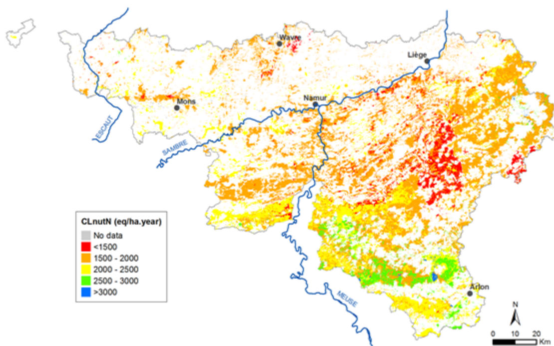
Figure 15 Critical loads of nutrient nitrogen for forests, CLNut(N)- Steady State model
