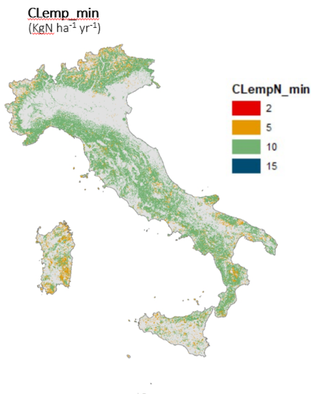
Figure 18 CL_{emp\_min} minimum value for receptor ecosystems map
