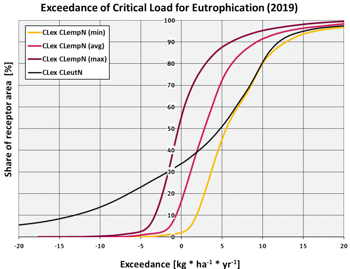
Figure 17 CL exceedance in Germany
