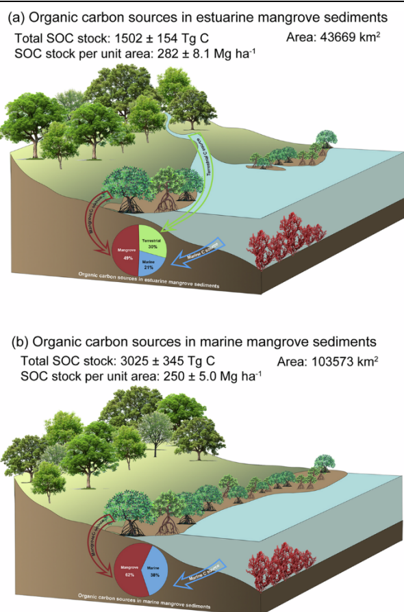
Figure 3: A conceptual diagram summarizing organic carbon (OC) sources in estuarine and marine mangrove sediments.
