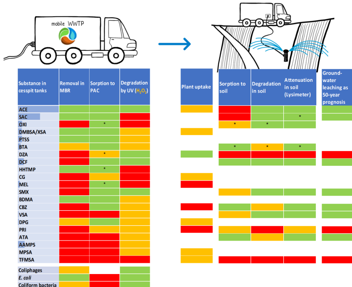
Figure 3: Qualitative retention of organic micropollutants (OMPs) and microbial water quality indicators (red = low, yellow = medium, green = high) given for the processes in the multi-barrier system. Substances are sorted according to MBR feed concentrations of the individual OMPs and bar graphs in the first column illustrate semi-quantitative concentrations in wastewater from single-household cesspits. Degradation by UV marked in yellow is related to addition of H_2O_2 inducing an advanced oxidation process. A high uptake by plants is marked in red, a low uptake in green.
