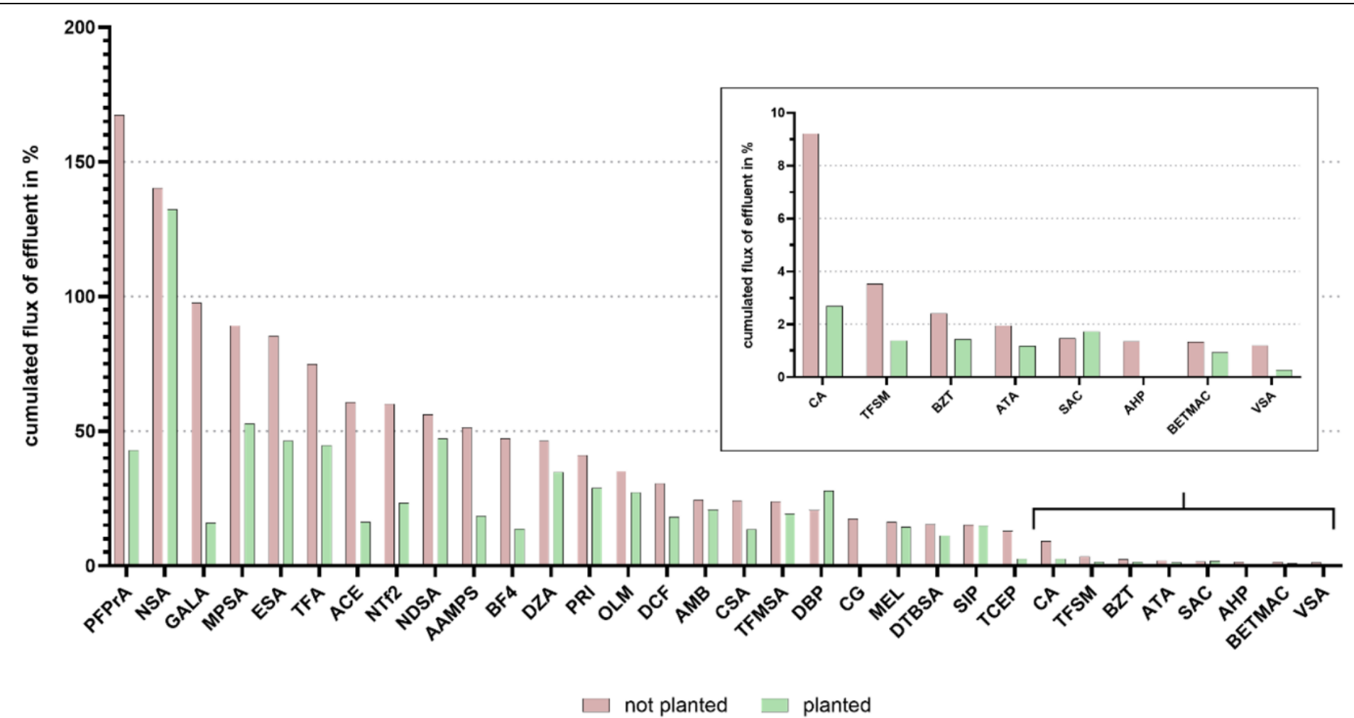
Figure 2: Cumulative load of PM substances in the effluent of the lysimeters (60 cm) over the operating period of 9 months in relation to the cumulative load in the inflow in %, for planted (green) and non-planted (red) lysimeters.
