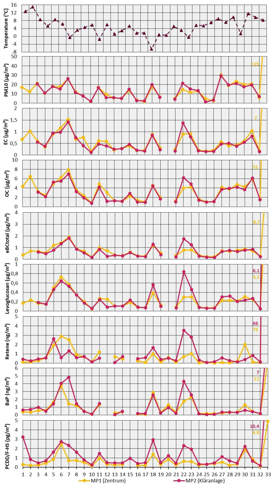
Figure S 1: Compilation of selected wood combustion tracers in the short-term (weekend) samples in Thalheim/Erzgeb. at MP1 (center) and MP2 (wastewater treatment plant)
