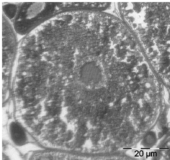
Figure 2: Zebrafish ( Danio rerio ) oocytes in maturation
