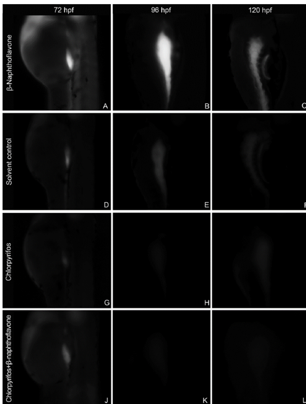
Figure 33: In vivo localization of EROD activities in zebrafish ( Danio rerio ) embryos after exposure to chlorpyrifos in various scenarios I
