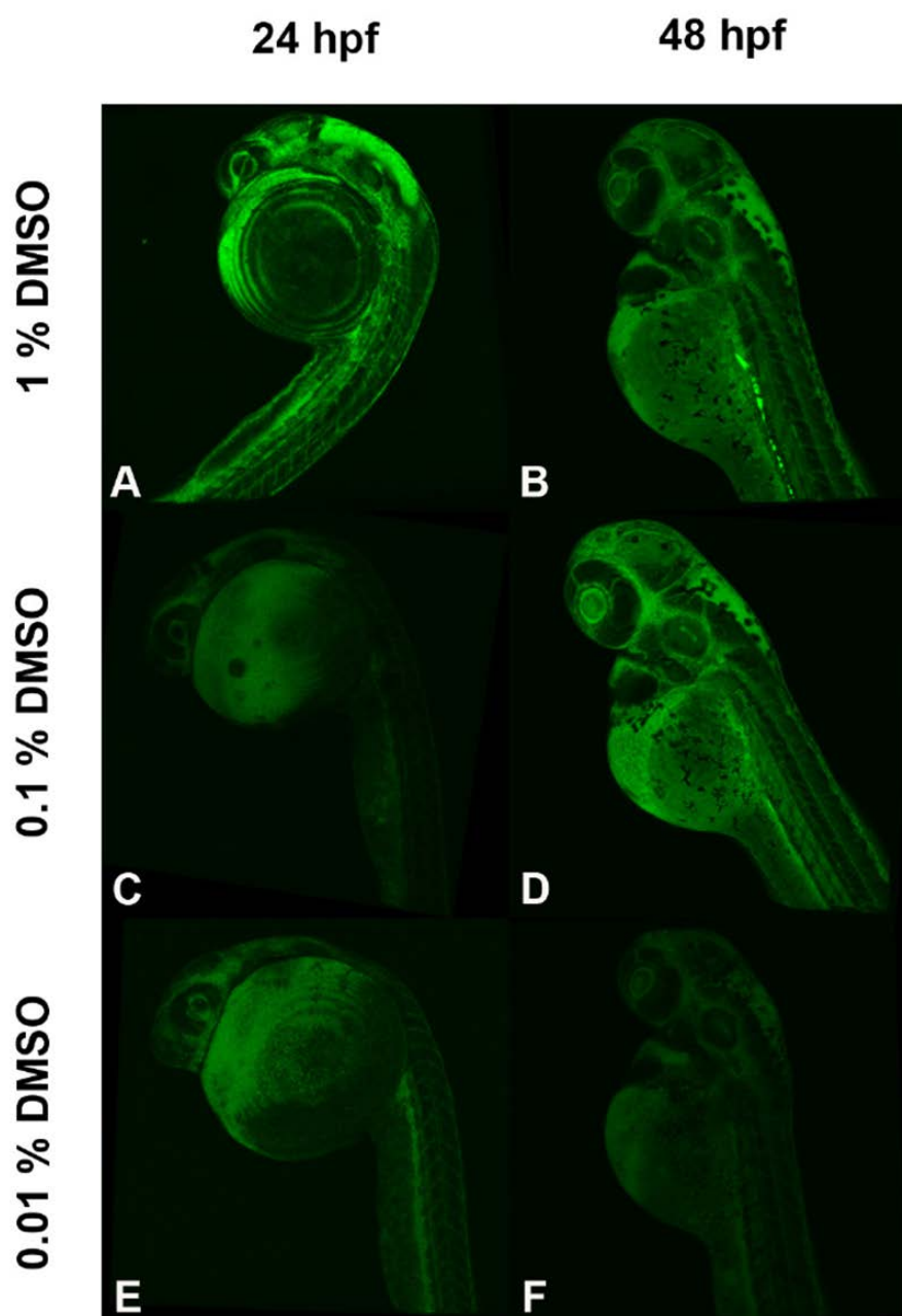
Figure 23: Cross-section and composite 3D surface images of zebrafish ( Danio rerio ) embryos after exposure to 2,7-dichlorofluorescein II
