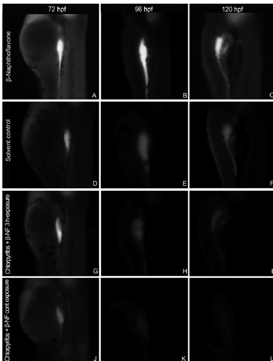
Figure 35: In vivo localization of EROD activities in zebrafish ( Danio rerio ) embryos after exposure to chlorpyrifos in various scenarios III
