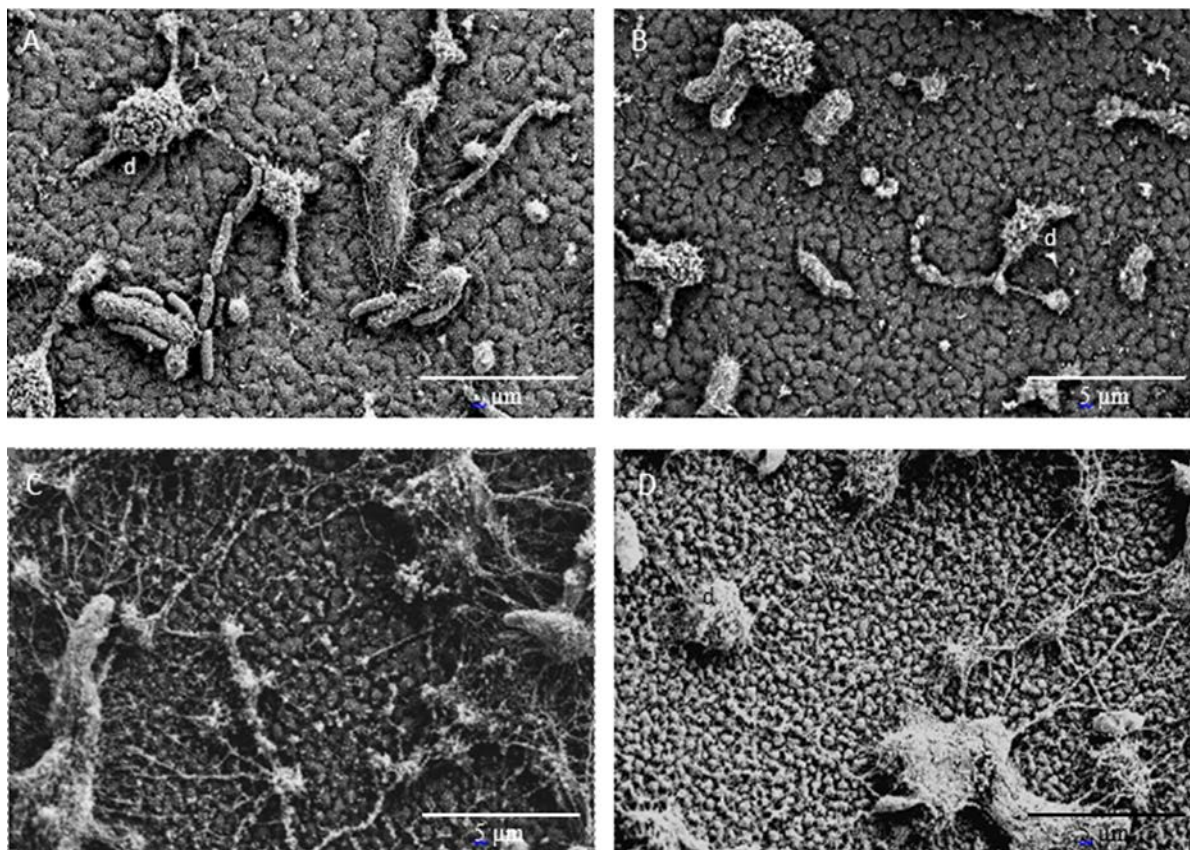
Figure 6: Surface of the zebrafish ( Danio rerio ) chorion
