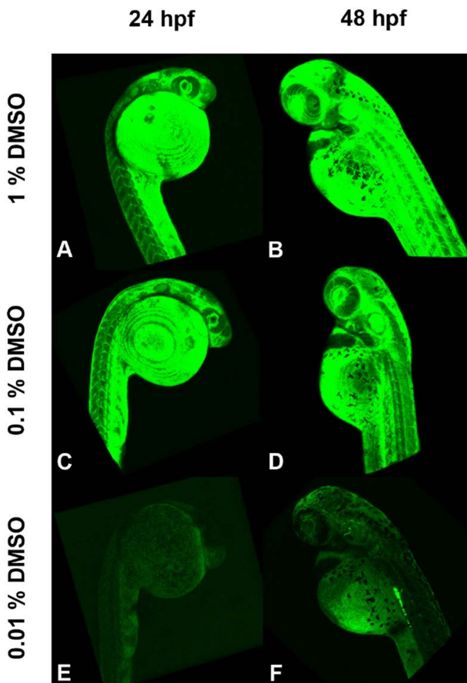
Figure 21: Composite 3D surface confocal laser images of zebrafish ( Danio rerio ) embryos
