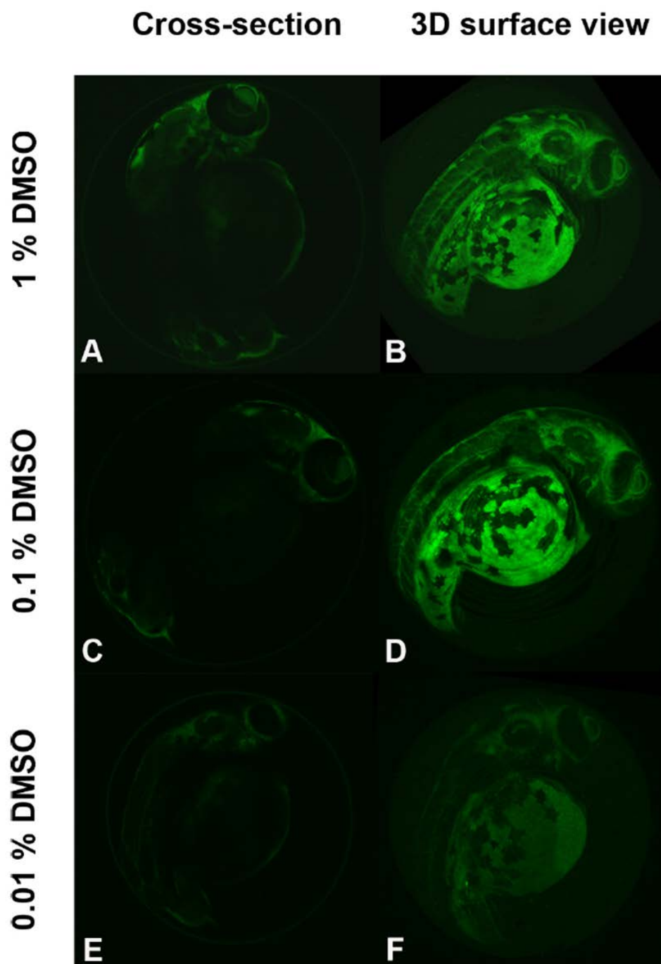
Figure 22: Cross-section and composite 3D surface images of zebrafish ( Danio rerio ) embryos after exposure to 2,7-dichlorofluorescein I
