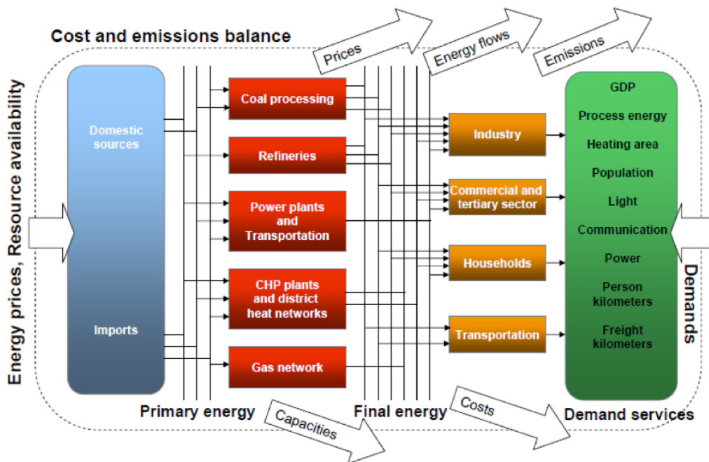
Figure 8: TIMES model structure
