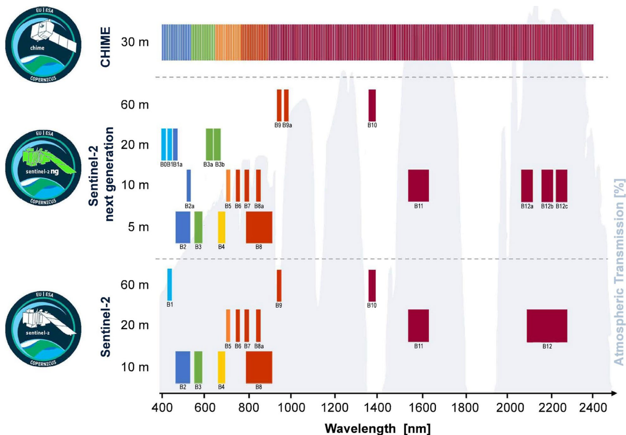
Fig. 2 Spectral and spatial configurations of Sentinel-2, S2NG and CHIME. Similarity of Sentinel-2 and S2NG bands reflects the key consideration of the mission on enhanced continuity, but also improved spectral information for new product provision. Continuous spectral coverage is represented by CHIME
