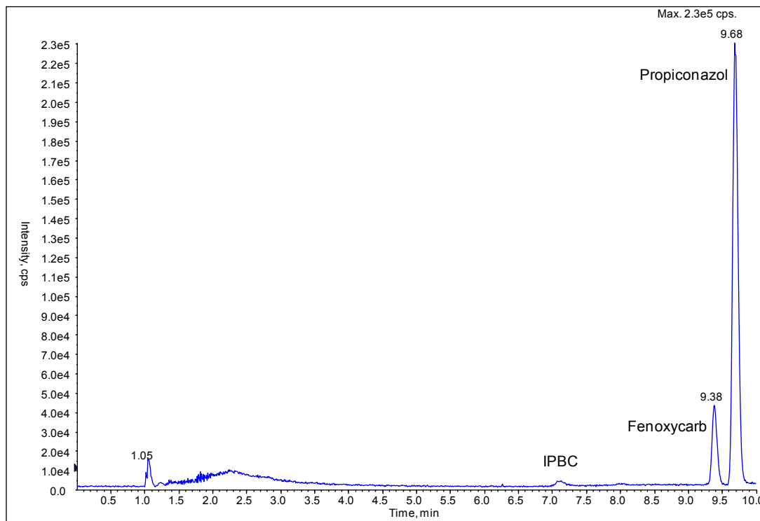
Fig. 4: Chromatogram of a standard solution of propiconazole, fenoxycarb and IPBC (each at 1 ng/l) after pre-concentration
