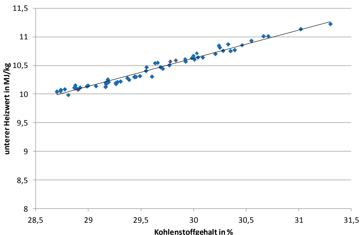
Figure 84: Relationship between carbon content and net calorific values, illustrated with the example of crude-lignite quality [x axis = Carbon content, in %; y axis = Lower net calorific value, in MJ/kg]
