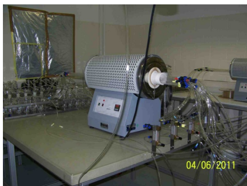
Figure 11: tube furnaces for combustion of methane to carbon dioxide and subsequent trapping in NaOH-solution
