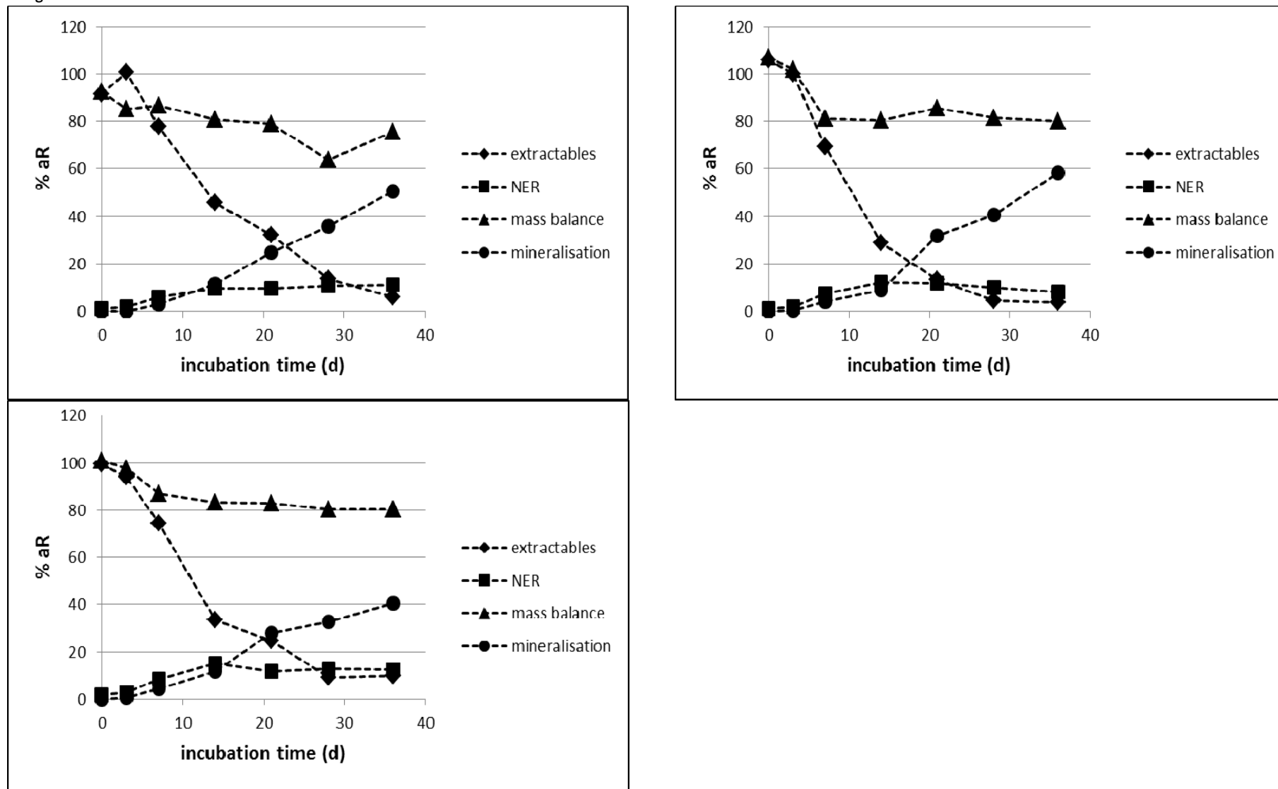
Figure 18: Radioactivity distribution for the transformation of ^{14}\text{C} -Salicylic acid in pig manure; sites: NRW_1p, NRW_2p, BAY_2p (from left to right)
