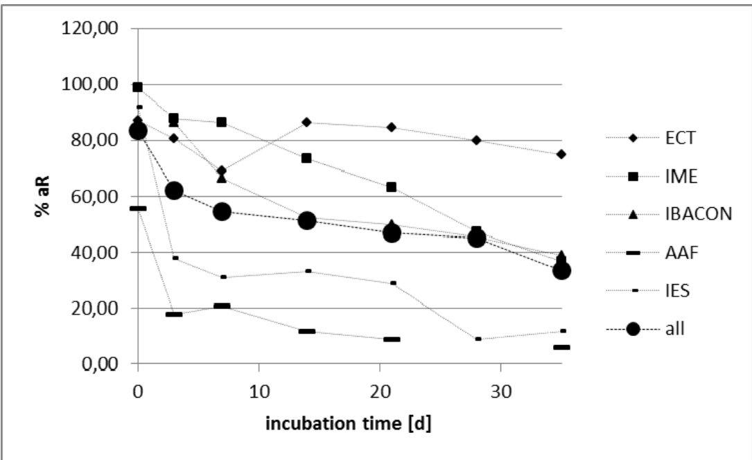
Figure 42: Comparison of extractable residues obtained from transformation of ^{14}\text{C} -Salicylic acid in cattle manure for the participants (means of each and of all) of the ringtest. The amount of radioactivity [% applied radioactivity, % aR] per sampling interval is given as arithmetic mean.
