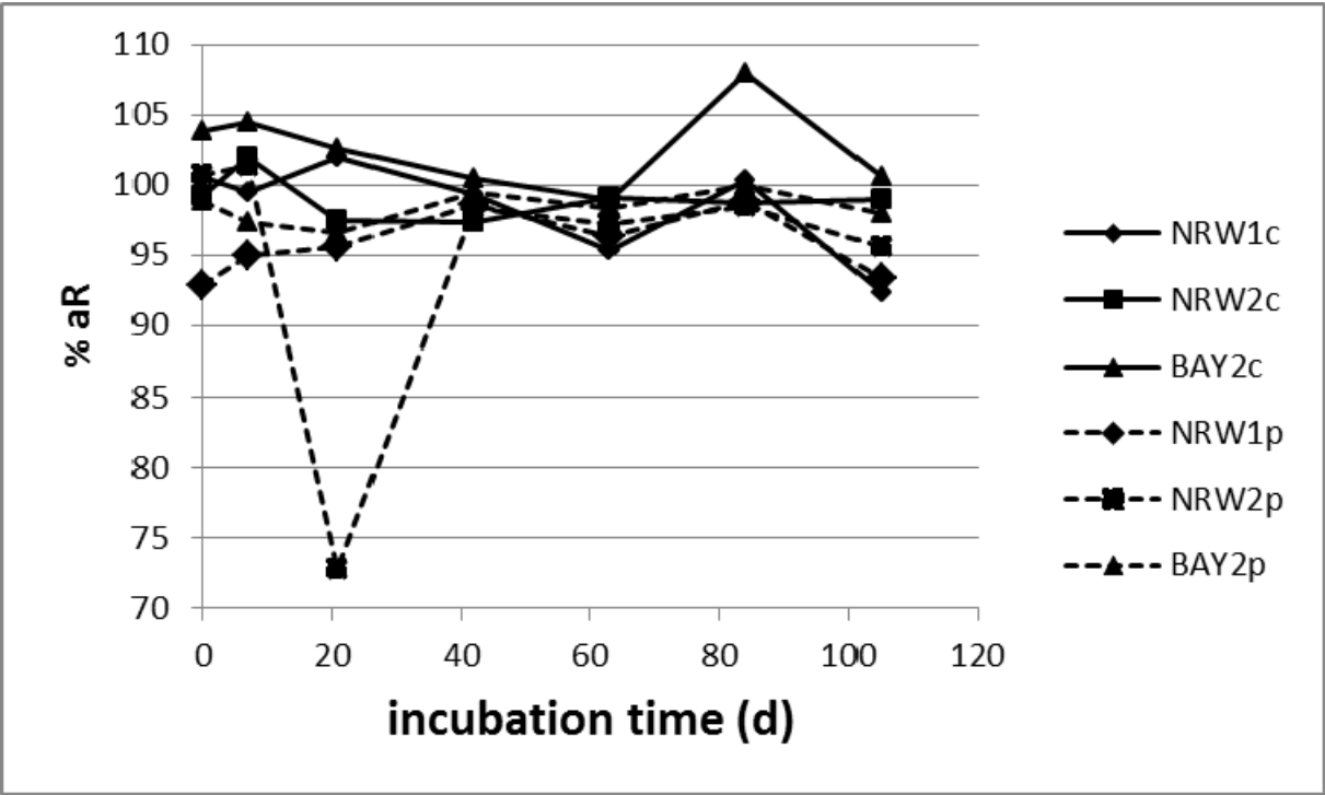
Figure 32: mass balance: Biocide B in cattle and pig manure
