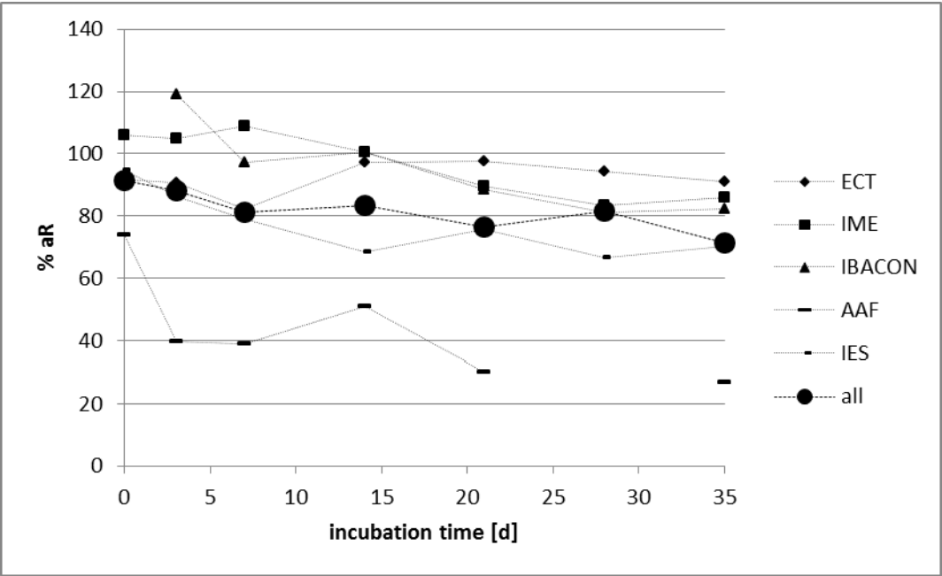
Figure 46: Mass balances for transformation of ^{14}\text{C} -Salicylic acid in cattle manure for all participants (means of each and of all) of the ringtest. The amount of radioactivity [% applied radioactivity, % aR] per sampling interval is given as re-transformed mean.
