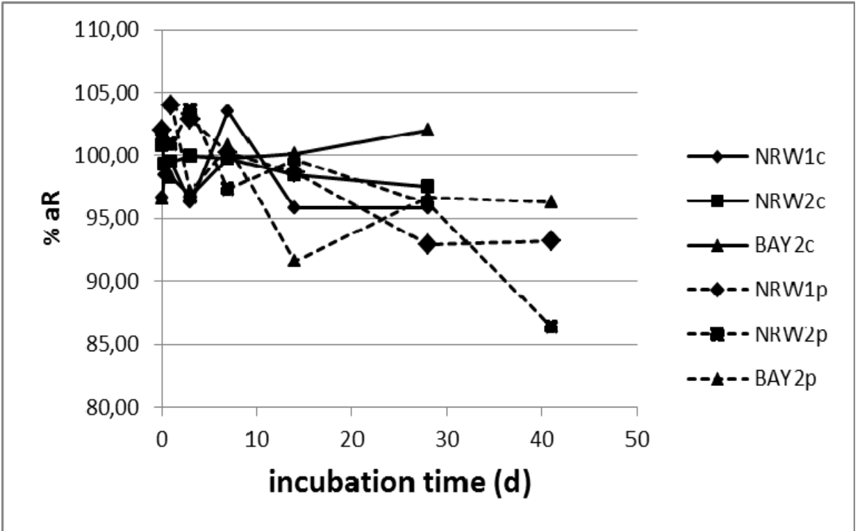
Figure 27: Mass balance: Paracetamol in cattle and pig manure
