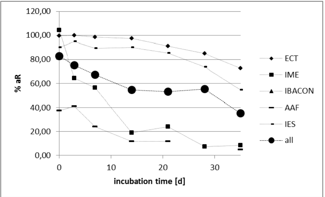
Figure 43: Comparison of extractable residues obtained from transformation of ^{14}\text{C} -Salicylic acid in pig manure for the participants of the ringtest. The amount of radioactivity [% applied radioactivity, % aR] per sampling interval is given as arithmetic mean.
