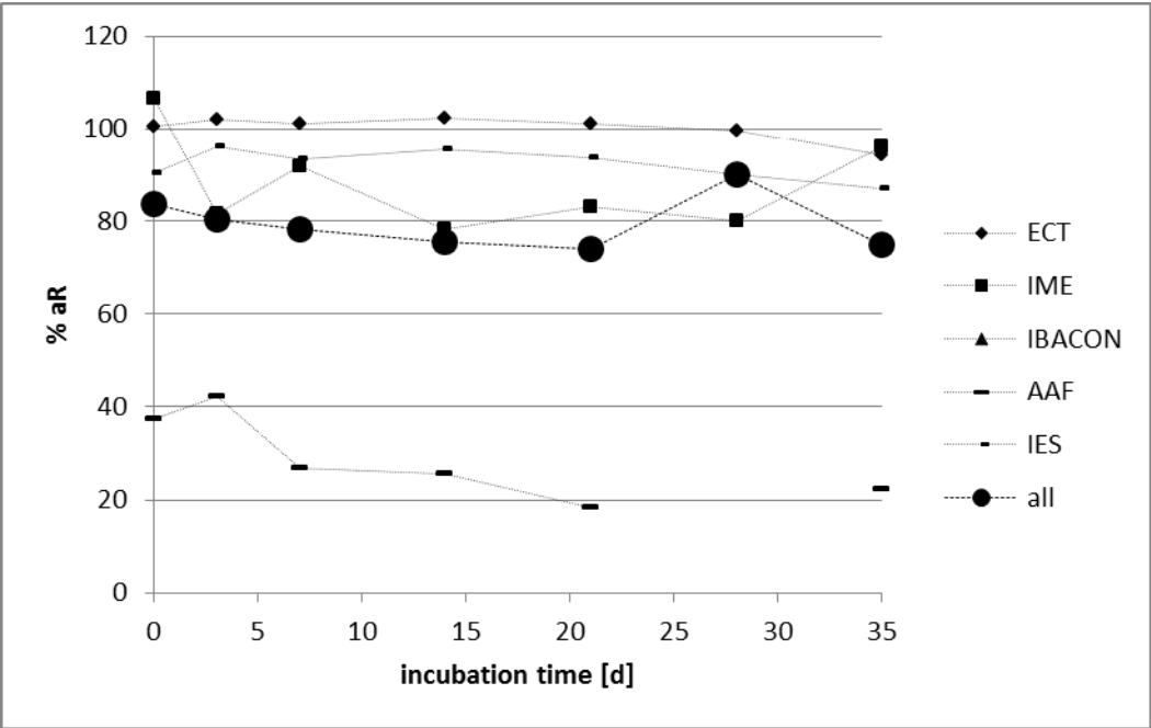
Figure 47: Mass balances for transformation of ^{14}\text{C} -Salicylic acid in pig manure for all participants of the ringtest. The amount of radioactivity [% applied radioactivity, % aR] per sampling interval is given as re-transformed mean.
